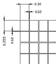
DETAIL A 20:1
