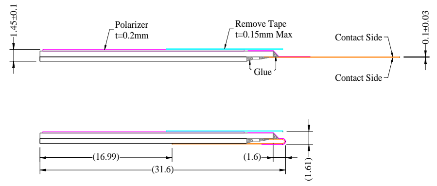
(Reference Mechanical Design)
