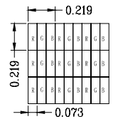
MAIN LCD DOTS DETAIL(20:1)
