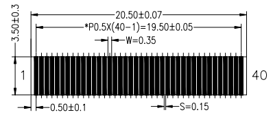
DETAIL B SCALE 4:1 TYPE:FH19S-40S-0.5SH(51)
