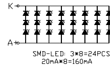
LED circuit
