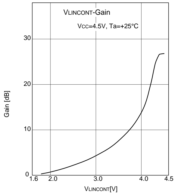
LINGCA Gain Control
