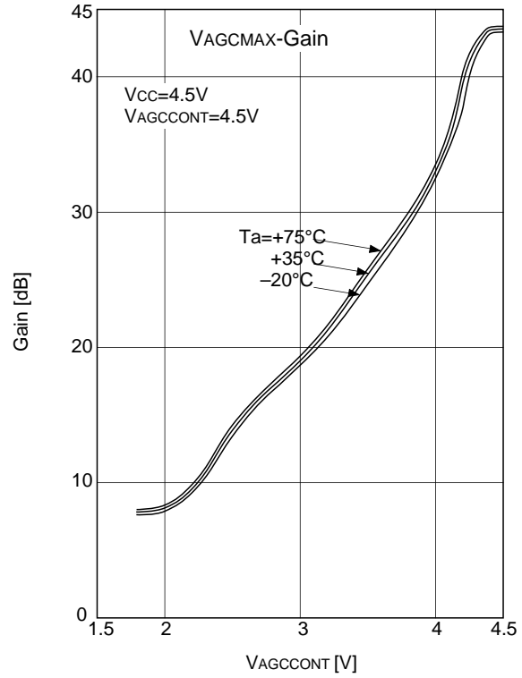
AGC CONT Control Temperature Characteristics
